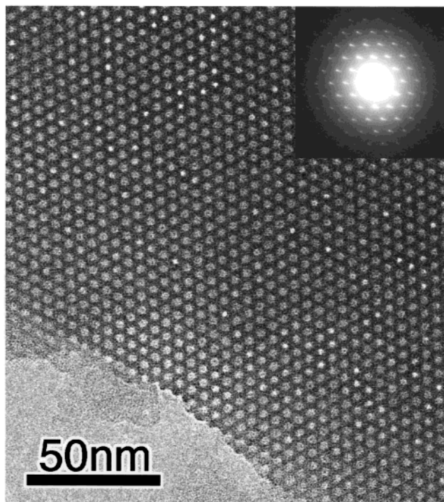
Figure 3. Transmission electron micrograph and electron diffraction pattern (inset) of the mesoporous material with 2D-hexagonal symmetry.
