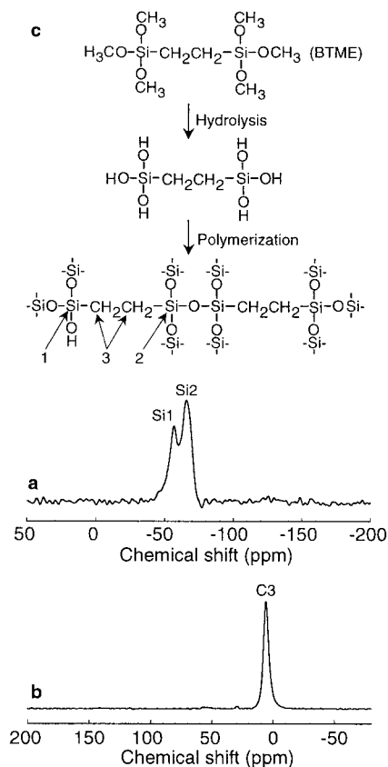
Figure 5. (a) ^{29}\text{Si} MAS NMR and (b) ^{13}\text{C} CP MAS NMR spectra of the mesoporous material with 2D-hexagonal symmetry. (c) Chemical reaction path for the formation of the organic–inorganic hybrid network structure with peak assignments of the NMR spectra.
